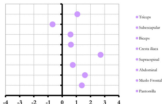
Score-Z Pliegues
